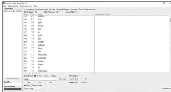
Figure 1: Display of Word List and Word Tokens of AntConc 3.4.3
