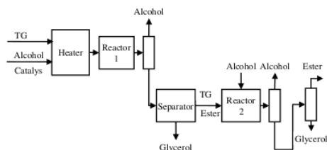
Gambar 2. Proses biodiesel sistem continuous
