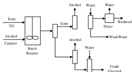
Gambar 1. Proses biodiesel sistem batch
