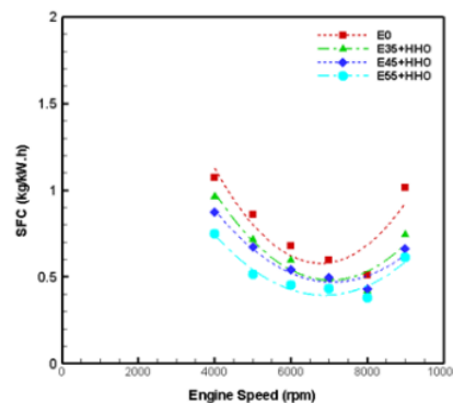
Figure 5. Variety of Specific FC to engine speed
