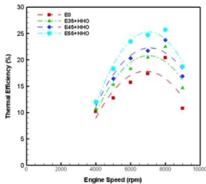
Figure 6. Variety of Efficiency to engine speed.
