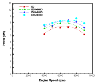
Figure 3. Variety of power to engine speed
