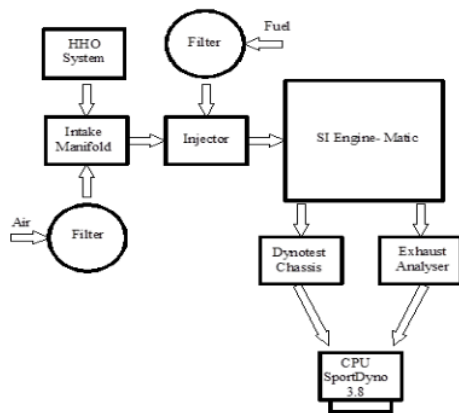
Figure 2. SI Engine Matic set-up.
