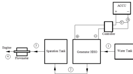
Figure 1. Schematic of component HHO gas system.
