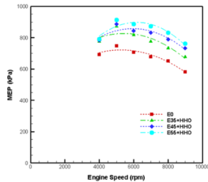
Figure 4. Variety of Mean pressure to engine speed.
