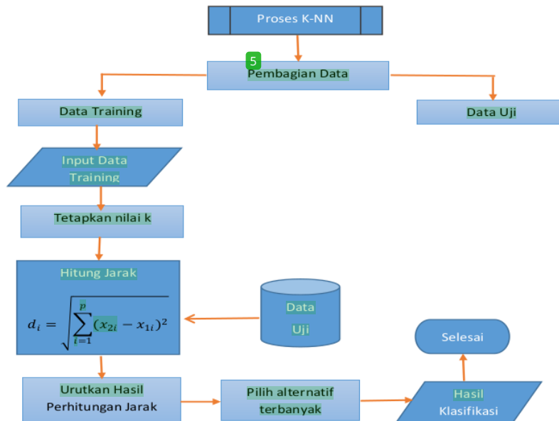
Gambar 1. Diagram Alir Metode K-Nearest Neighbors (K-NN)
